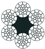
6x26 WS+FC
